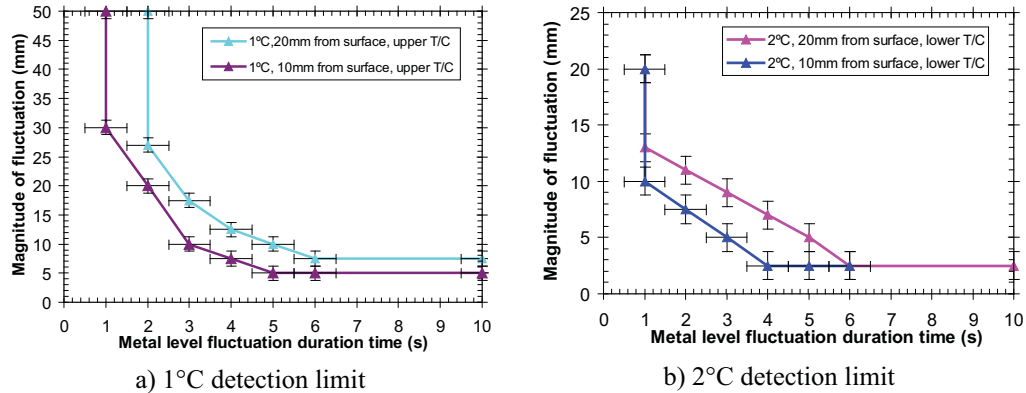
Fig. 8. Effect of TC distance beneath hot-face on critical detectable level fluctuation at lower TC
