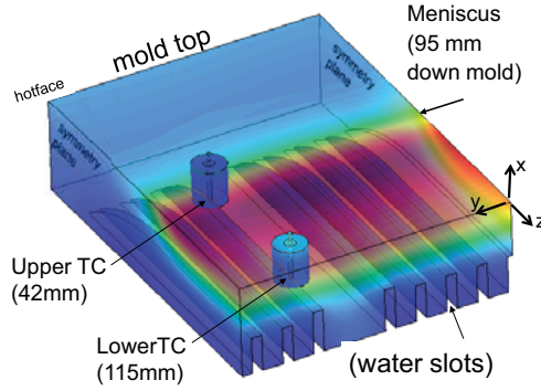
Fig. 1. Model domain and steady temperature distribution
