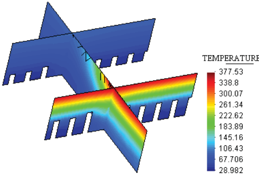
Fig. 3. Steady temperature contours ( ^{\circ}\text{C} ) in mold sections for base mold level (95mm down mold)
